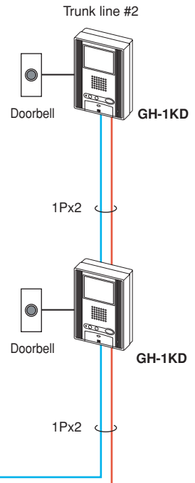
Station-to-station wiring
